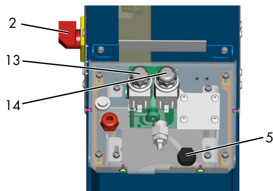
2 Main switch 13 Valve V1 5 Oil filling opening 14 Valve V2 002
