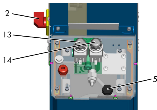
2 Main switch 5 Oil filling opening 13 Valve V1 14 Valve V2
